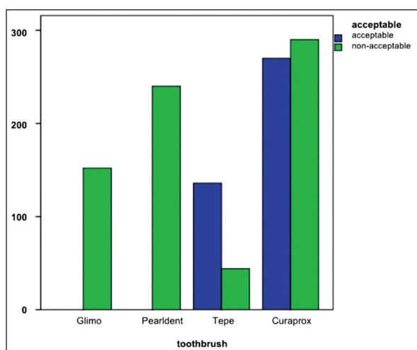
FIGURE 2: Graphical representation of the distribution of bristle end morphologies, evaluated according to Silverstone and Featherstone classification.
